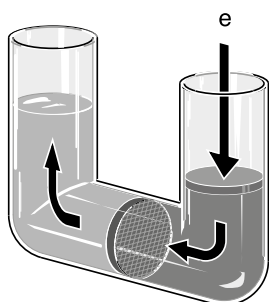
Osmose inverse
